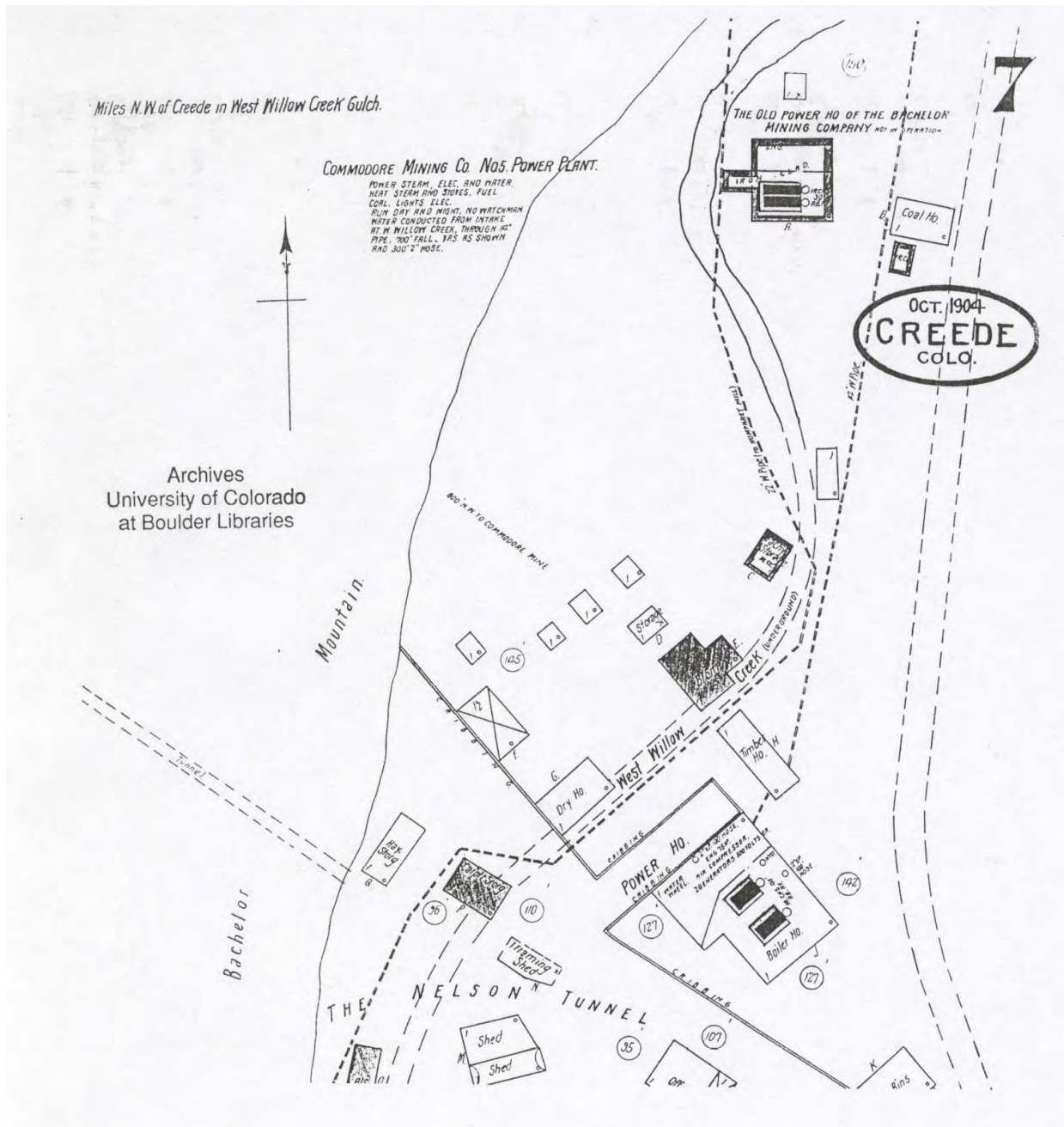
Figure 1. 1904 Sanborn Fire Insurance map of Commodore Mine Surface Plant, from Mining the Amethyst Vein , 104. None of the buildings shown on this map are extant today, though the foundation of the Bachelor power plant at top remains (Site Feature 3).
